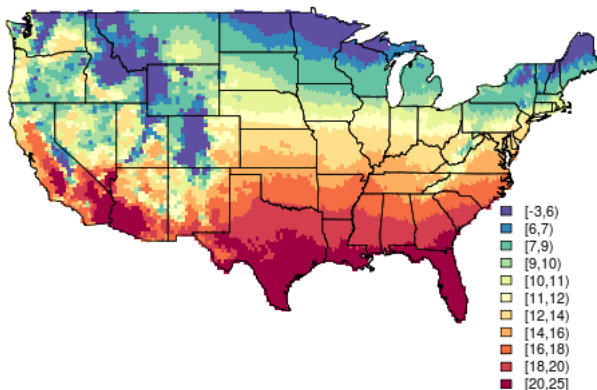
Average Air Temperature
