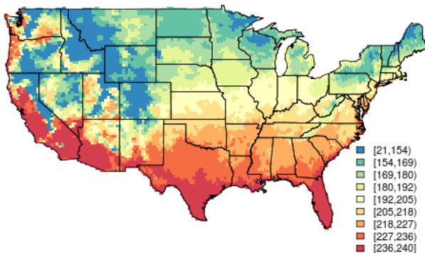
Length of the growing season
